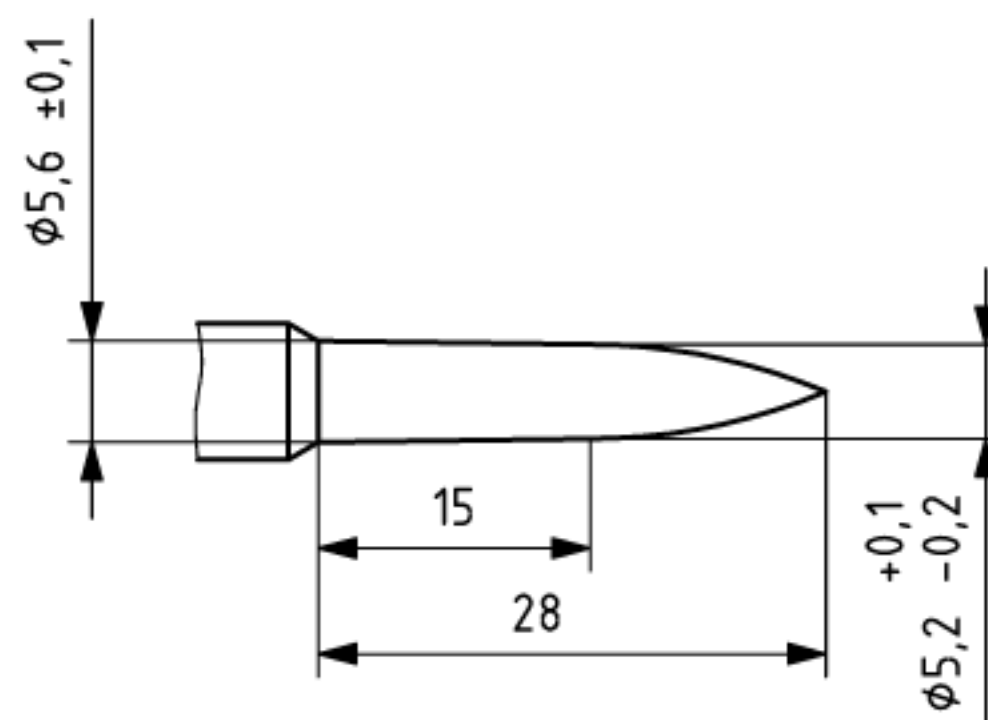
Figure 4 — Dimensions of the closure-piercing device
