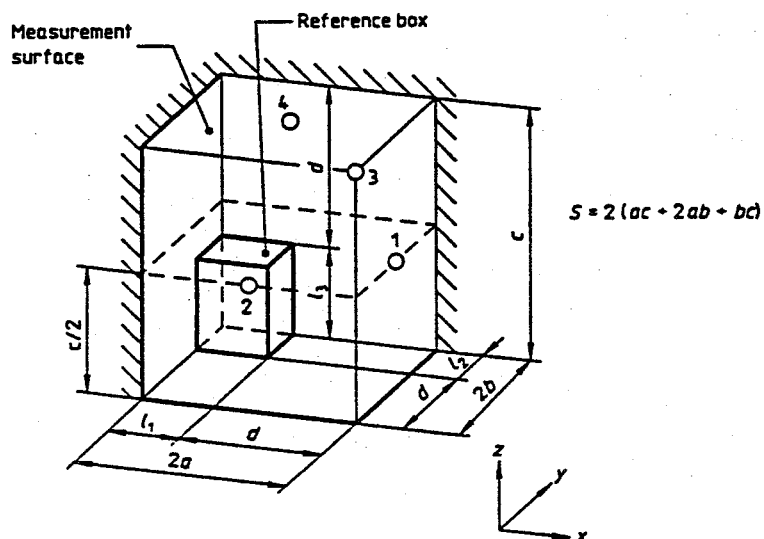
Figure C.8 — Measurement surface (parallelepiped) with four microphone positions for floor-standing appliances placed against two walls
