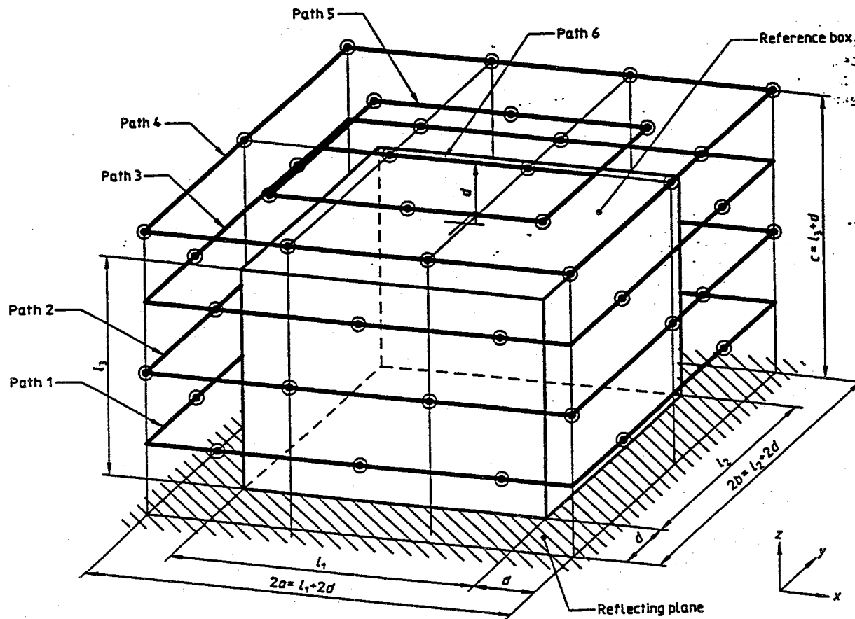
Figure C.6 — Example of a measurement surface and microphone positions (paths) for a large machine (4d < l_1 \leq 7d, d < l_2 \leq 4d, 2d < l_3 \leq 5d)
