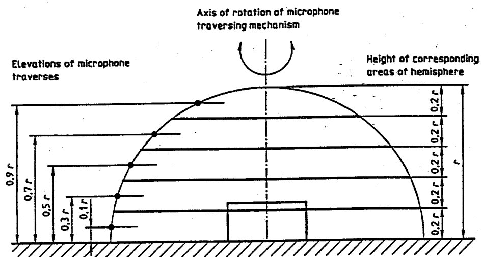
Figure B.4 — Coaxial circular paths in parallel planes for microphone traverses in a free field over a reflecting plane
