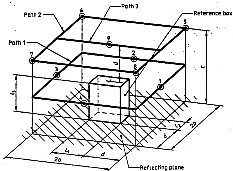
Figure C.2 — Example of a measurement surface and microphone positions (paths) for a small machine ( l_1 < d , l_2 < d , l_3 < 2d , where d is the measurement distance, normally 1 m)
