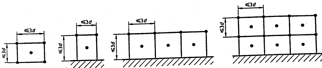
Figure C.1 — Procedure for fixing the specified microphone positions where a side of the measurement surface exceeds 3d
