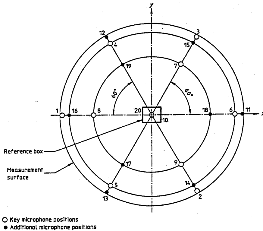
Figure B.2 — Microphone array on the hemisphere
