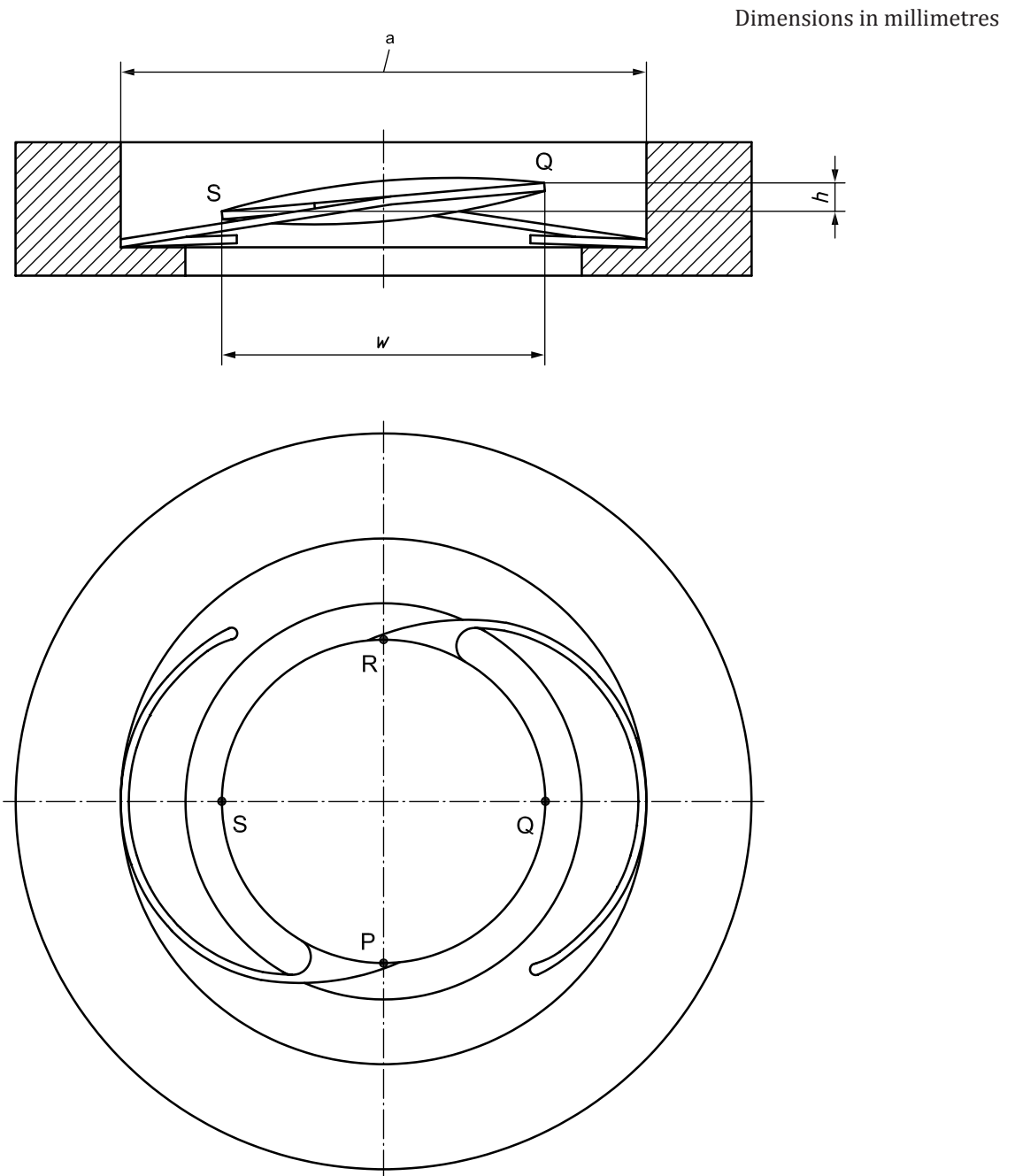
Figure D.2 — Determination of optic tilt
