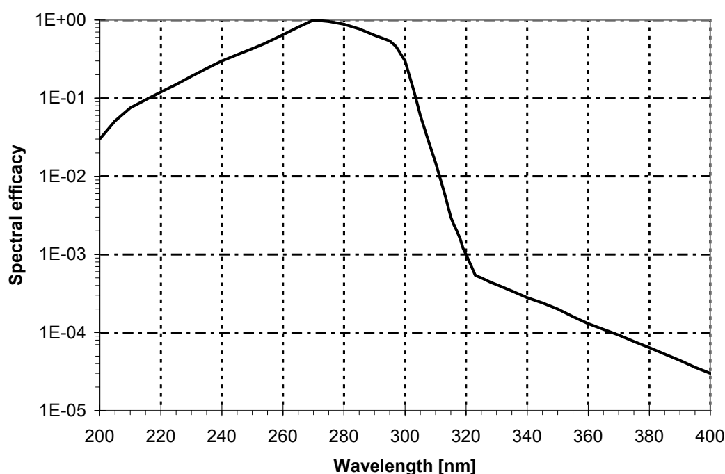
Figure 4.1 Spectral weighting function, S_{UV}(\lambda) , for actinic UV hazard for skin and eye.
