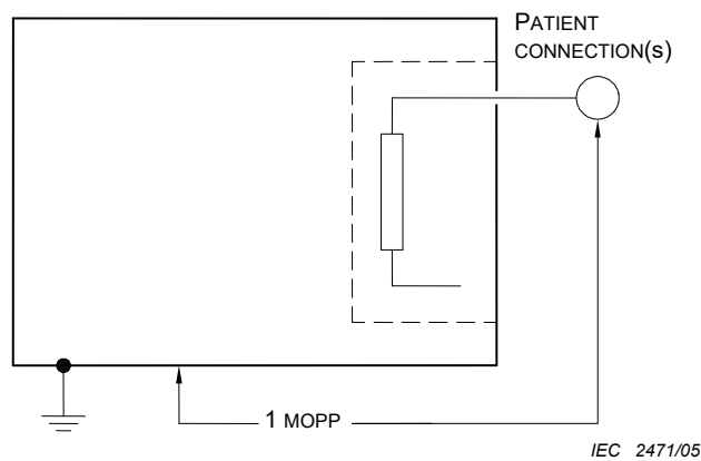
Figure J.6 – Insulation example 6
