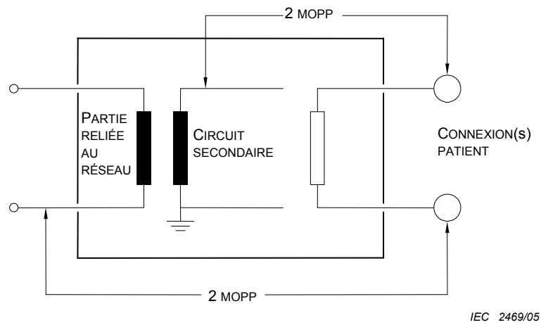
Figure J.5 – Isolation, exemple 5
