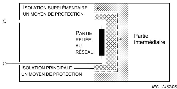
Figure J.3 – Isolation, exemple 3
