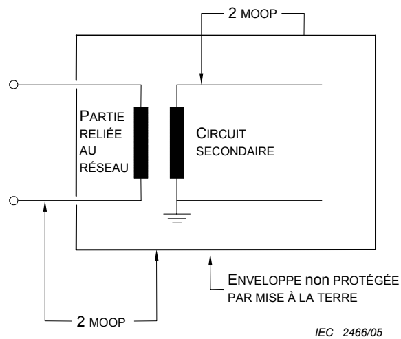
Figure J.2 – Isolation, exemple 2
