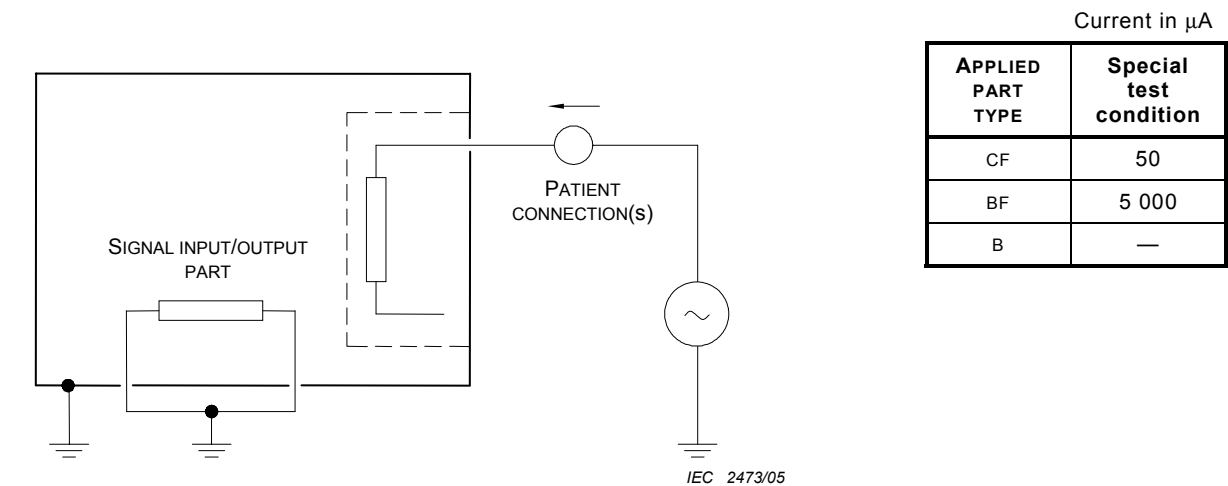
Figure K.2 – ME EQUIPMENT with an F-TYPE APPLIED PART (simplified Figure 16) (see 8.7.4.7 b))
