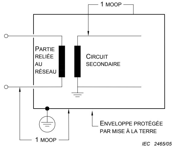
Figure J.1 – Isolation, exemple 1
