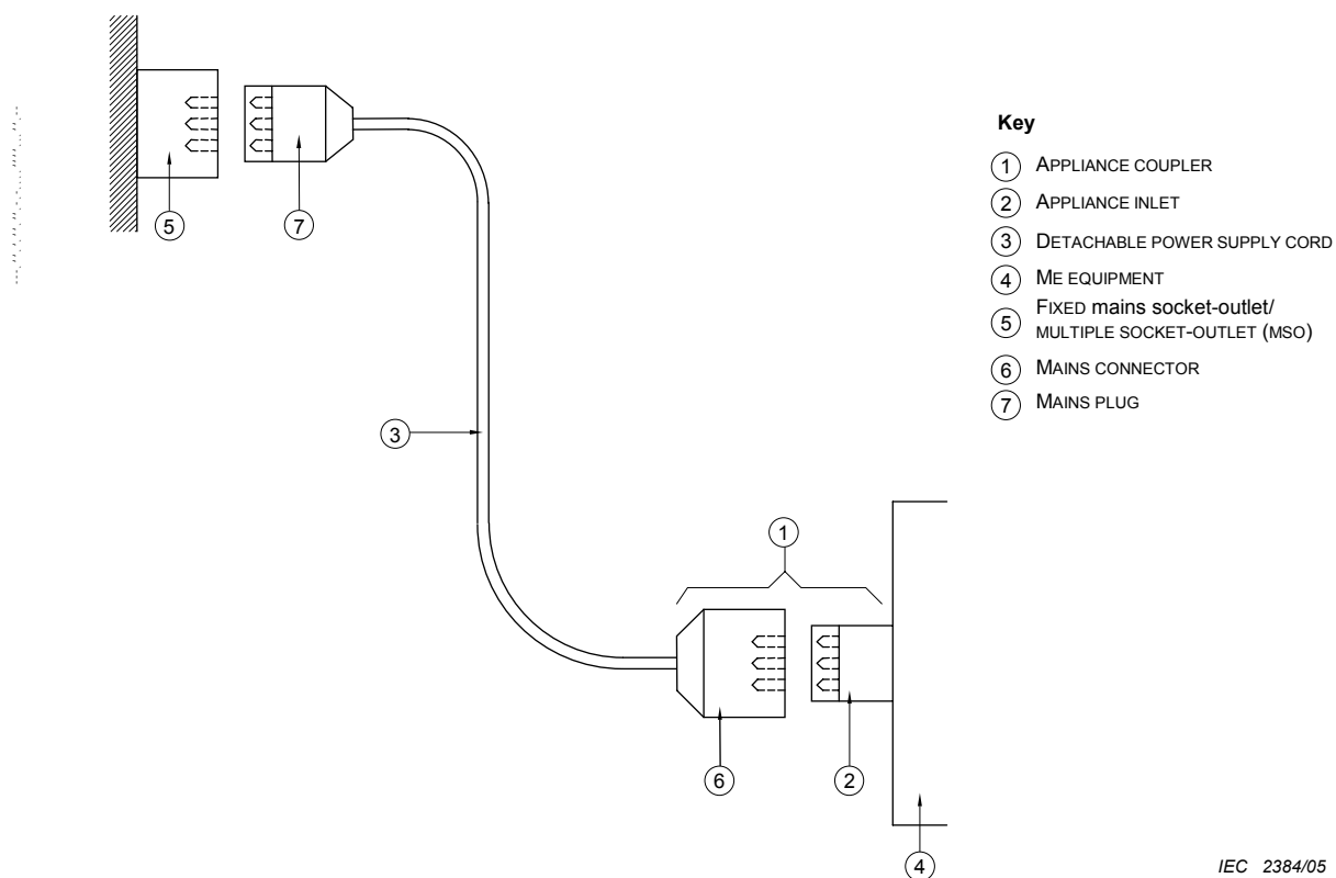
Figure 1 – Detachable mains connection (see definitions)
