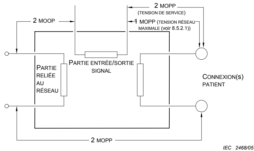
Figure J.4 – Isolation, exemple 4
