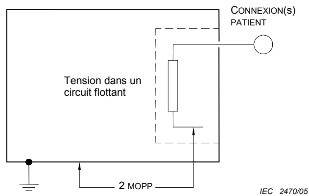
Figure J.6 – Isolation, exemple 6
