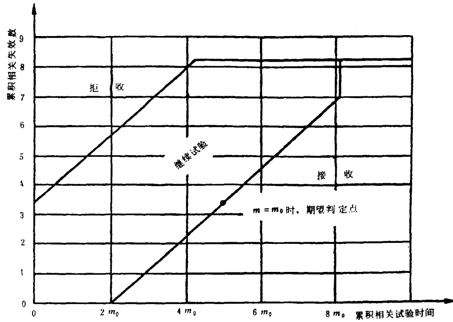
图 29 试验方案4:10 ( \alpha = 0.35 , \beta = 0.40 , D_m = 1.25 )
