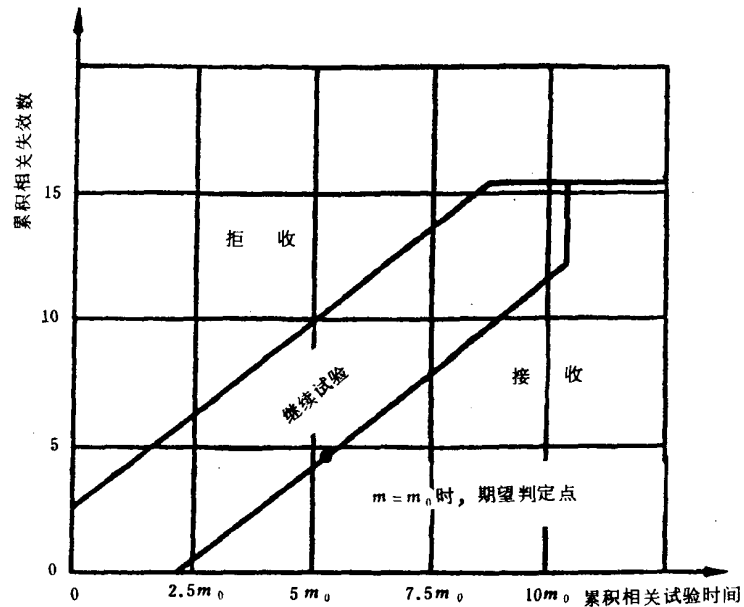
图 5 试验方案4:2 ( \alpha = 0.10 , \beta = 0.10 , D_m = 2.0 )
