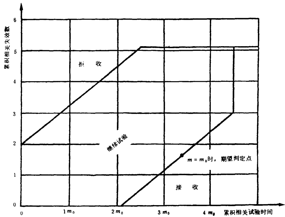
图 23 试验方案4:8 ( \alpha = 0.30 , \beta = 0.30 , D_m = 1.5 )
