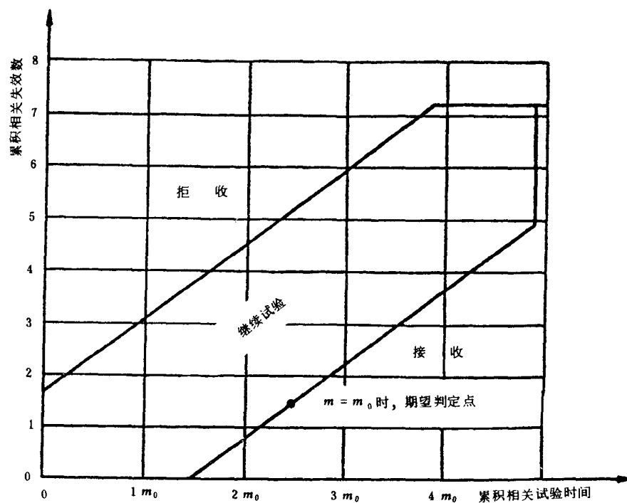
图 17 试验方案4:6 ( \alpha = 0.20 , \beta = 0.20 , D_m = 2.0 )
