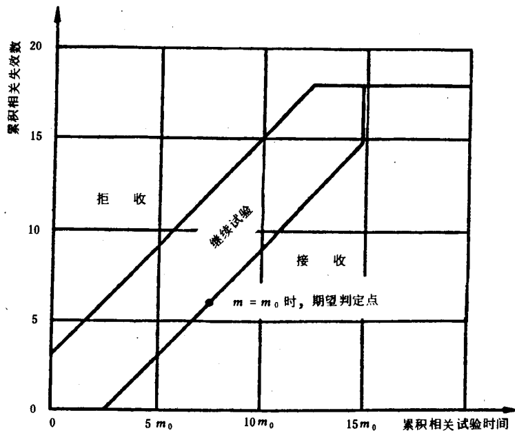
图 14 试验方案4:5 ( \alpha = 0.20 , \beta = 0.20 , D_m = 1.5 )
