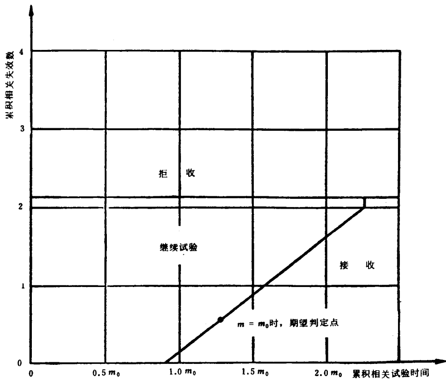
图 26 试验方案4:9 ( \alpha = 0.30, \beta = 0.30, D_m = 2.0 )
