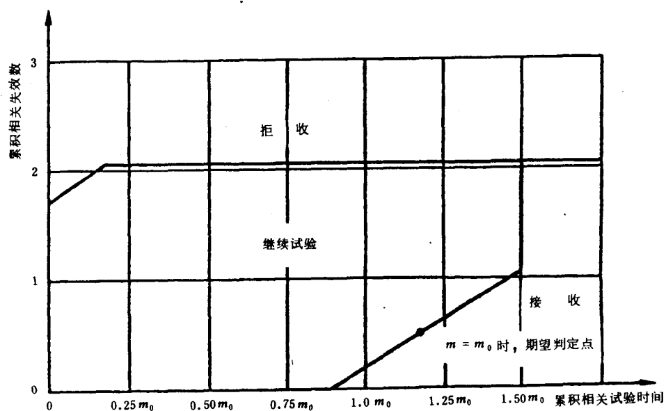
图 20 试验方案4:7 ( \alpha = 0.20 , \beta = 0.20 , D_m = 3.0 )
