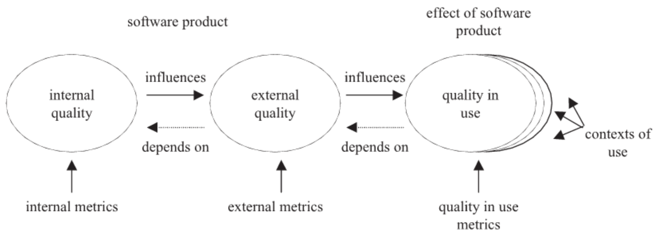
Figure 1 – Relationship between types of metrics
