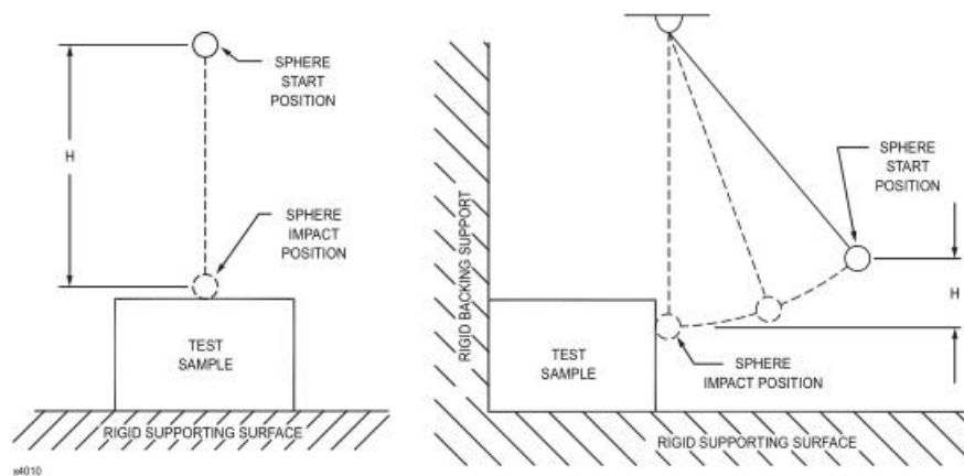
Impact Test
