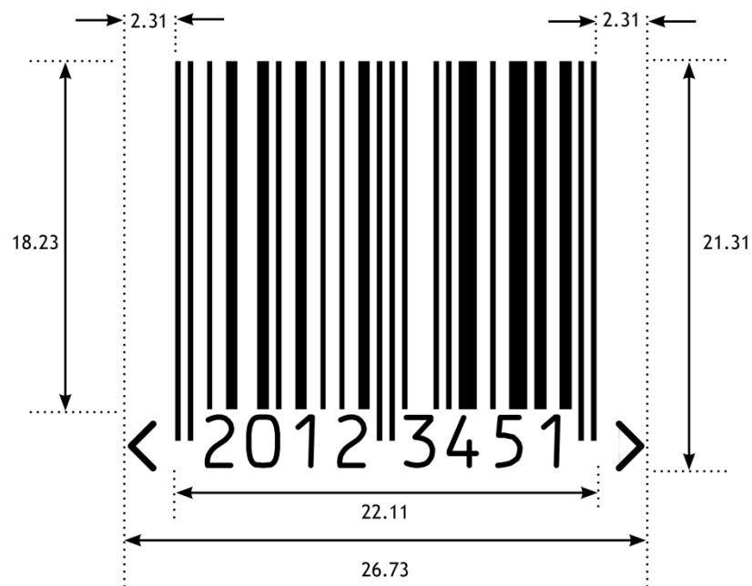
Figure 5.2.6.6-4. UPC-E barcode
