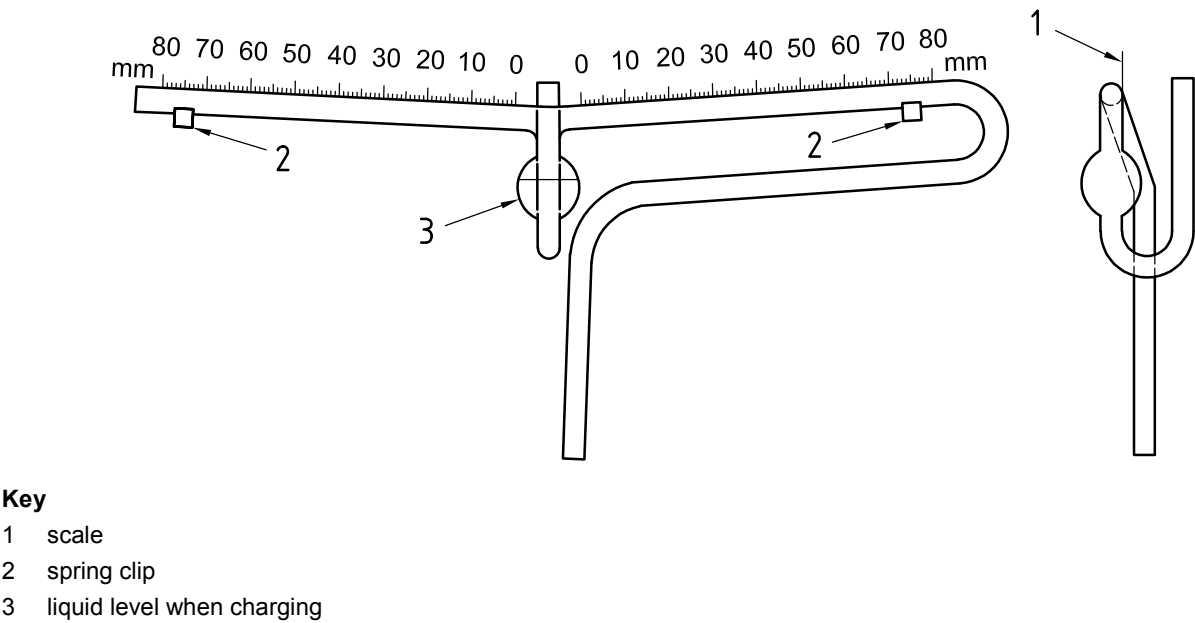
Figure F.4 — Parjo tube type A
