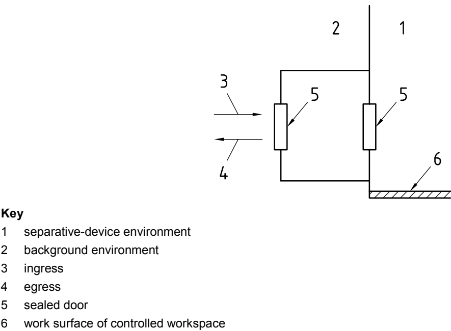
Figure D.3 — B1 transfer device
