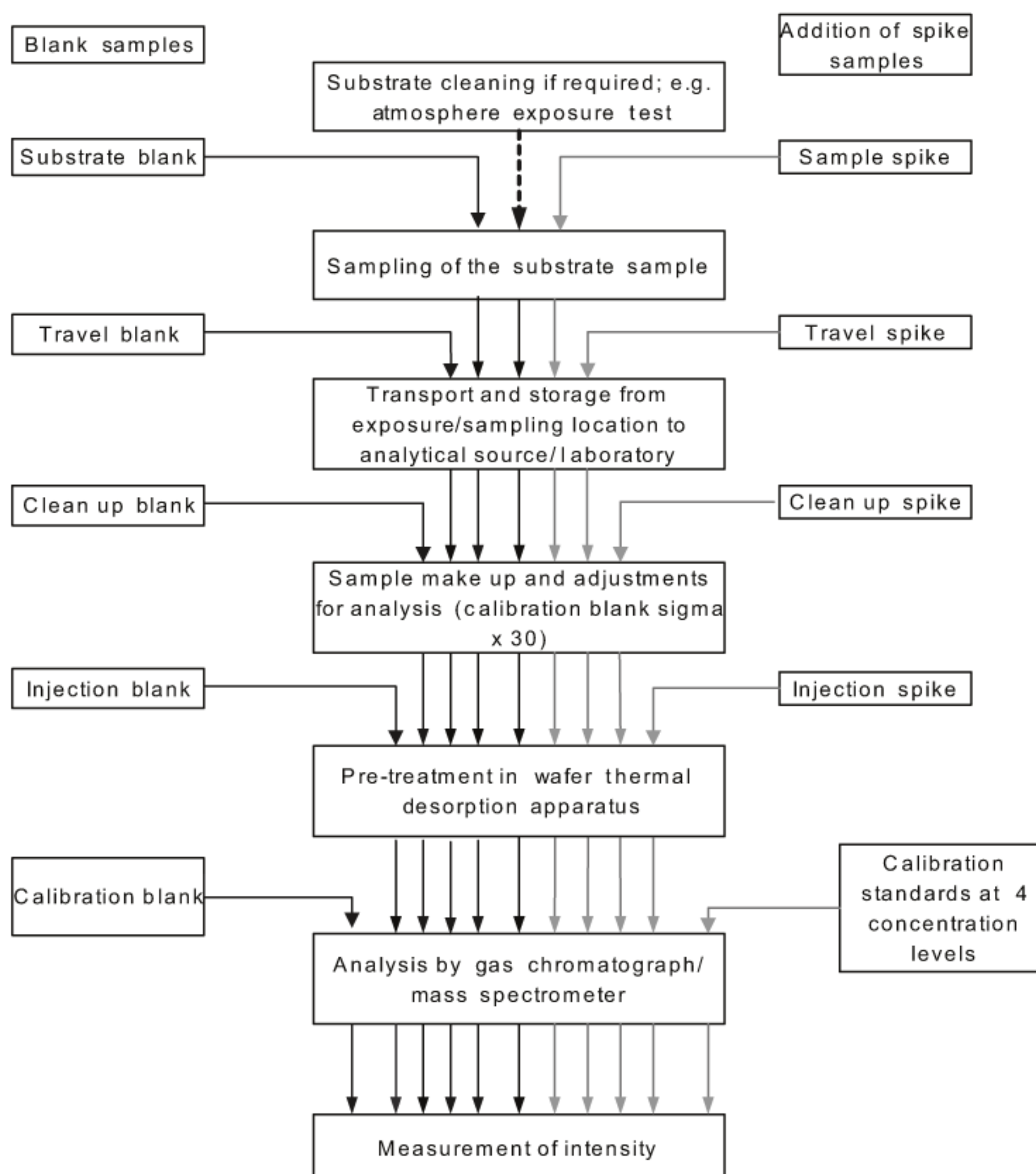
Figure D.4 — Analysis quality control flowchart using silicon wafer TD-GC/MS
