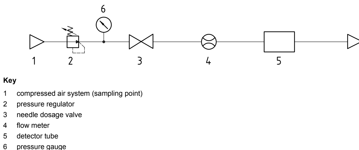
Figure D.1 — Example arrangement using gas detector tube method
