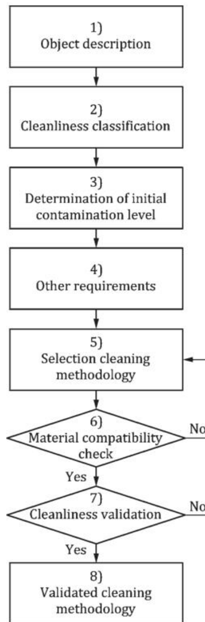
Figure 2 — Decision tree
