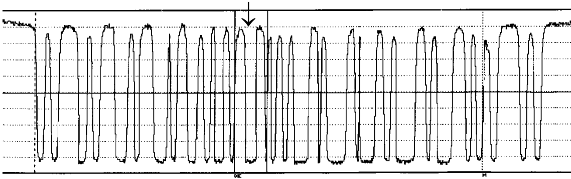
Figure 5.10.5.12-4. Scan Reflectance Profile of symbol with low decodability character
