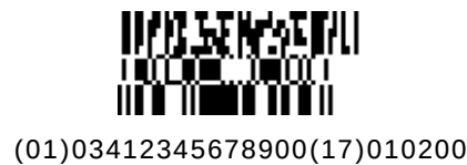
Figure 5.9.8-6. GS1 DataBar Stacked symbol with a two-column CC-A
