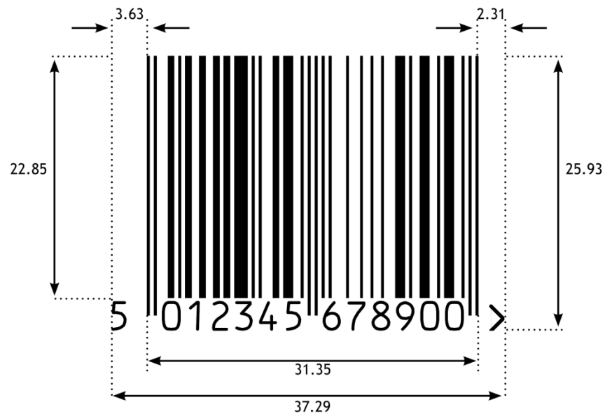
Figure 5.2.6.6-1. EAN-13 barcode
