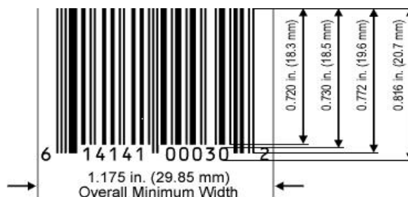
Figure 5.10.6.3-1. EAN/UPC symbol shown with minimum height and overall width dimensions for magnifications of 75 percent to 80 percent
