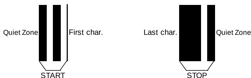
Figure 5.3.2.1.2-1. Start and stop patterns
