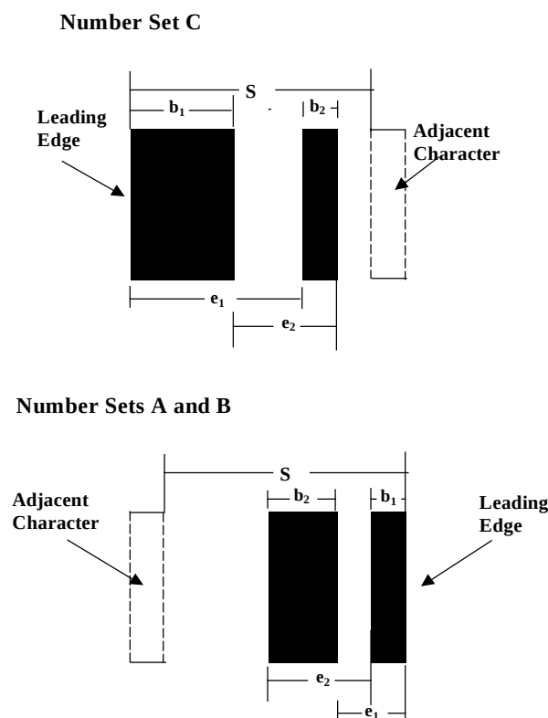
Figure 5.2.4-1. Symbol character decode measurements
