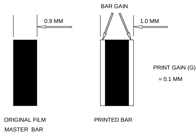
Figure 5.10.4.2.1-1. Example of bar width adjustment
