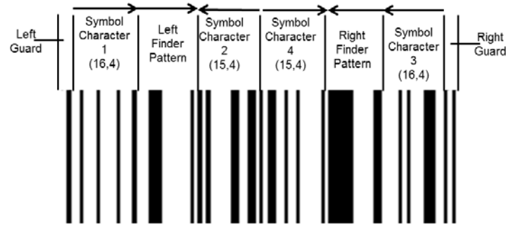
Figure 5.5.2.1-1. First group of GS1 DataBar symbols structure
