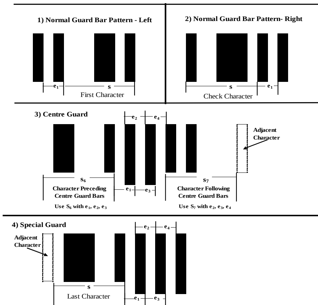
Figure 5.2.4-3. Auxiliary pattern measurements
