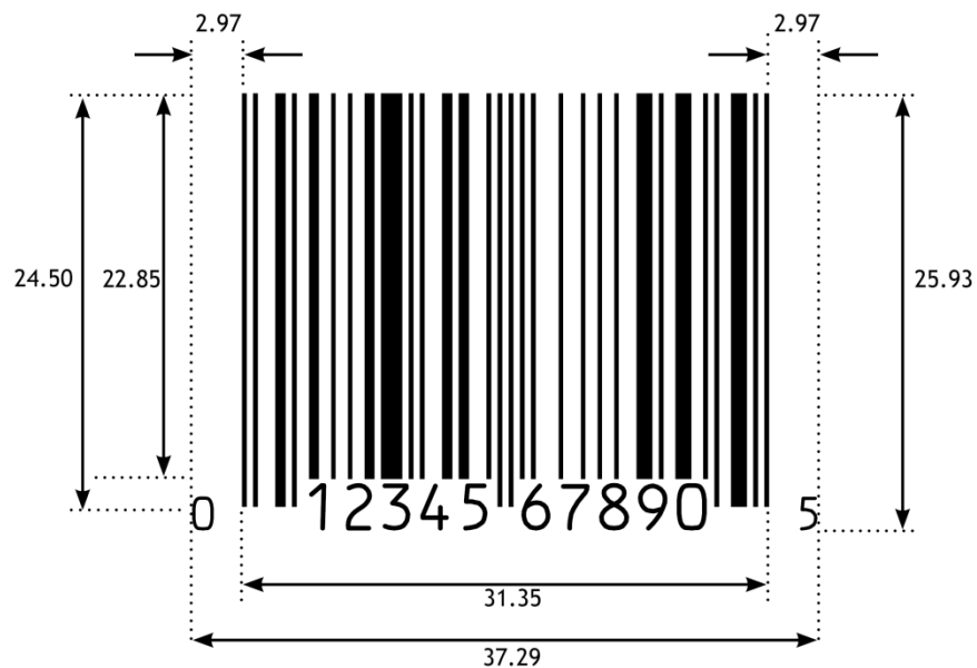
Figure 5.2.6.6-2. UPC-A barcode
