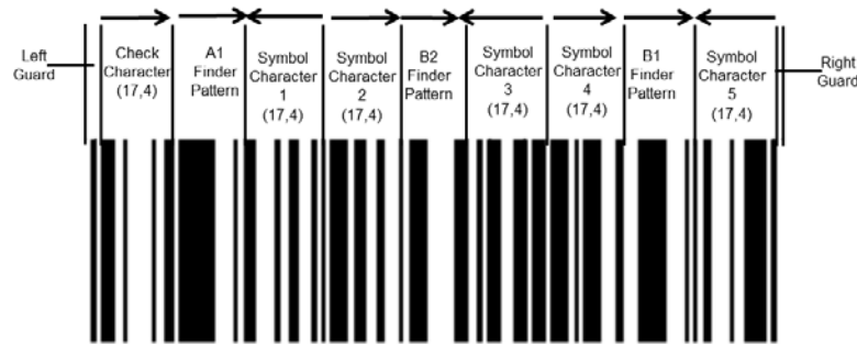
Figure 5.5.2.3-1. GS1 DataBar Expanded structure
