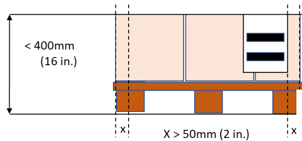
Figure 6.7.1.1-2. Symbol placement on pallets lower than 400 mm (16 inches)
