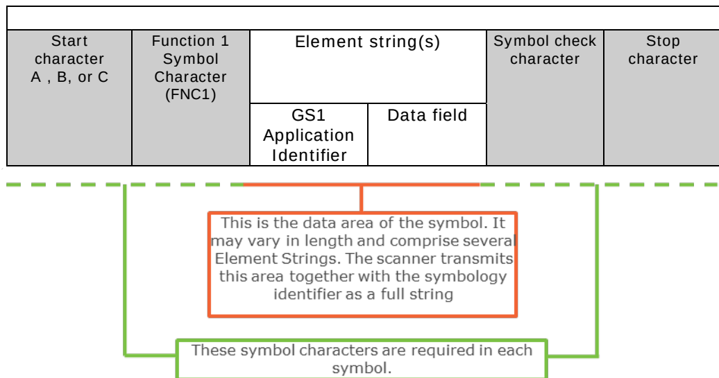
Figure 7.8.4-1. Example GS1-128 barcode structure
