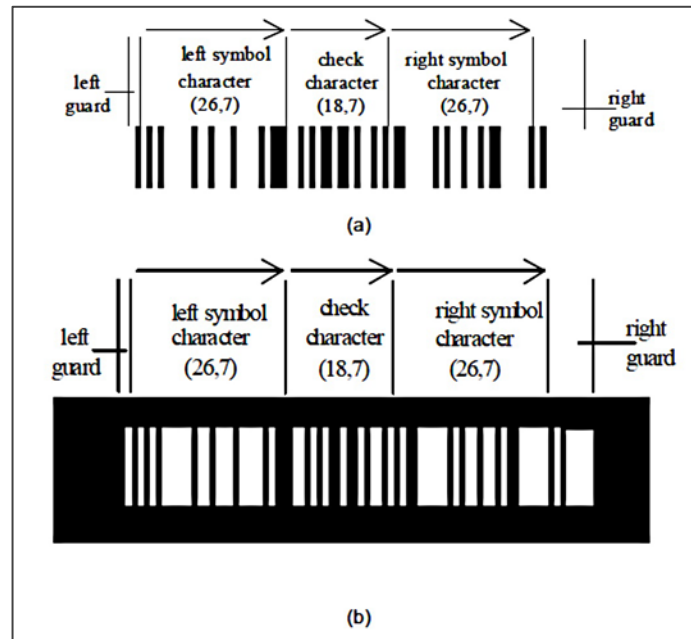
Figure 5.5.2.2-2. GS1 DataBar Limited barcode structure
