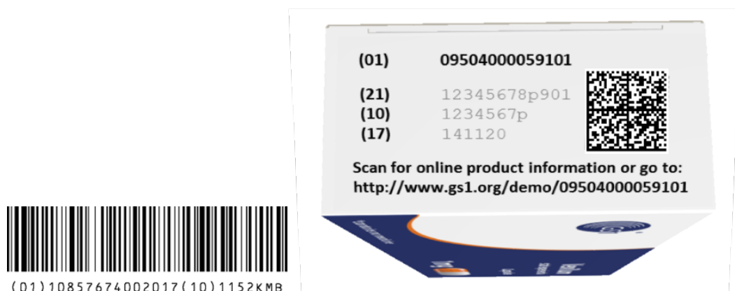
Figure 4.15.1-1. Preferred HRI format examples
