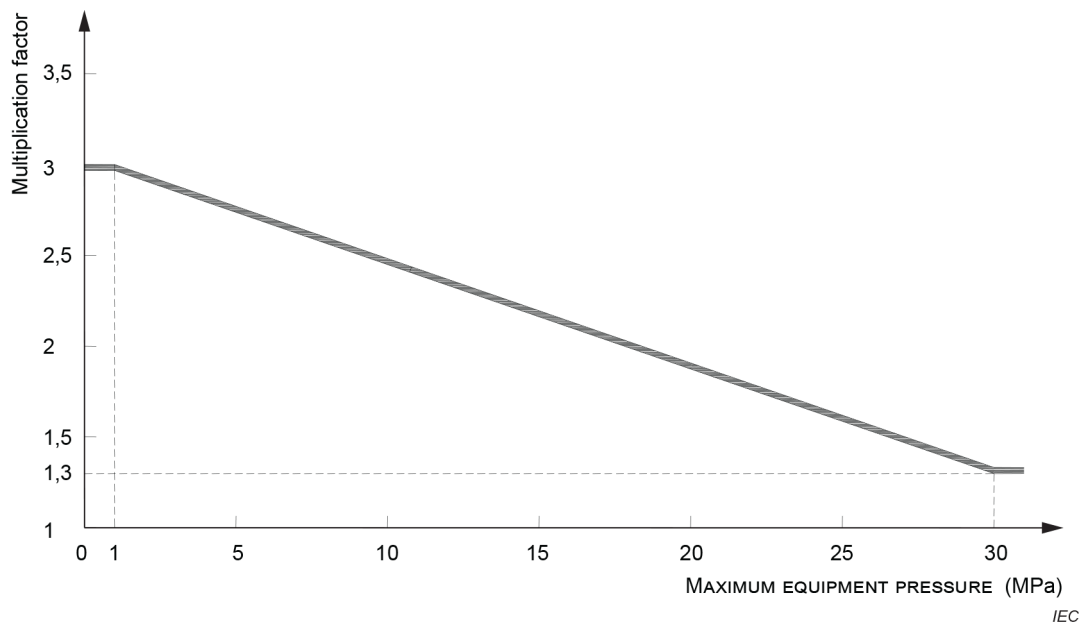
Figure 32 – Ratio between HYDRAULIC TEST PRESSURE and MAXIMUM PERMISSIBLE WORKING EQUIPMENT PRESSURE (see 9.7.5)
