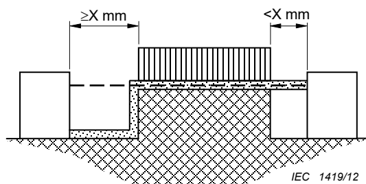
Figure 29 – CREEPAGE DISTANCE and AIR CLEARANCE – Example 8
