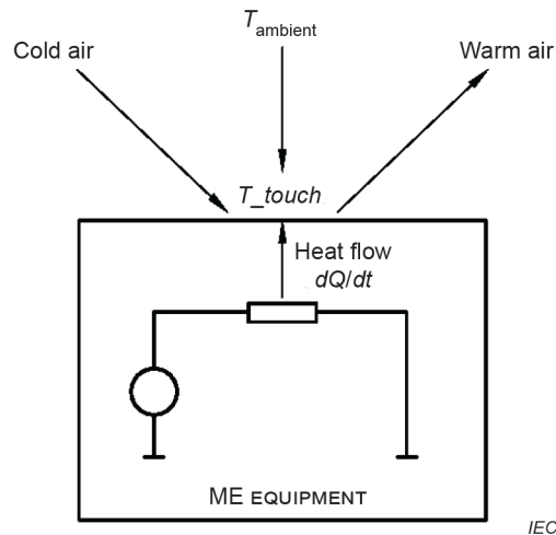
Figure A.22 – Maximum allowable temperature for surfaces and APPLIED PARTS at higher altitudes
