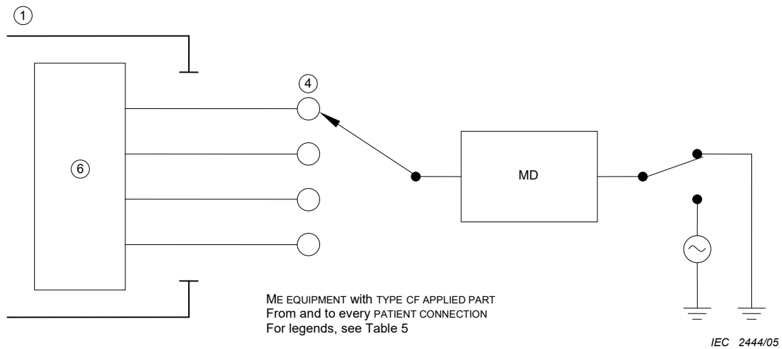
Figure E.3 – TYPE CF APPLIED PART
