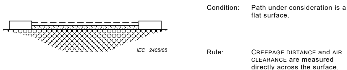
Figure 22 – CREEPAGE DISTANCE and AIR CLEARANCE – Example 1
