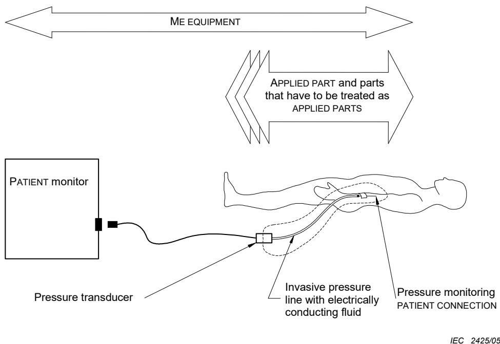
Figure A.3 – Identification of ME EQUIPMENT, APPLIED PARTS and PATIENT CONNECTIONS in a PATIENT monitor with invasive pressure monitoring facility
