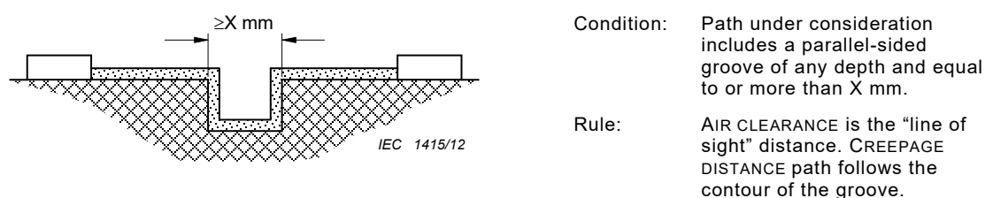
Figure 24 – CREEPAGE DISTANCE and AIR CLEARANCE – Example 3
