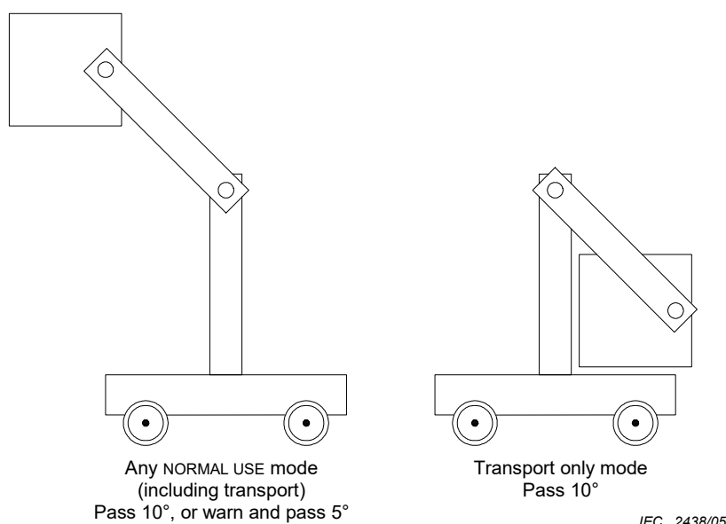
Figure A.15 – Instability test conditions
