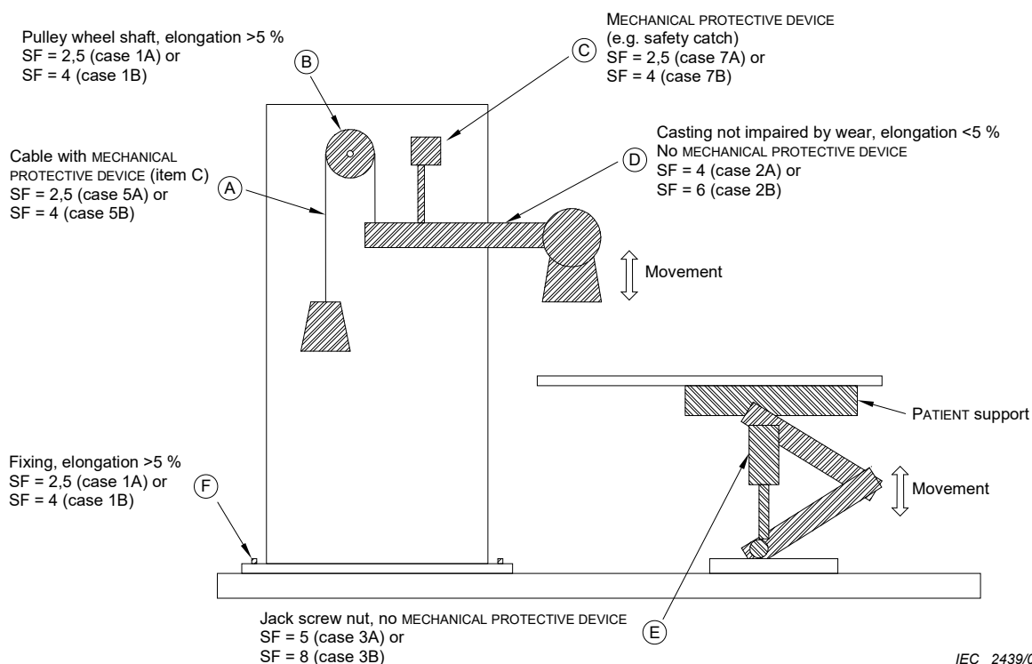
Figure A.16 – Example of determining TENSILE SAFETY FACTOR using Table 21
