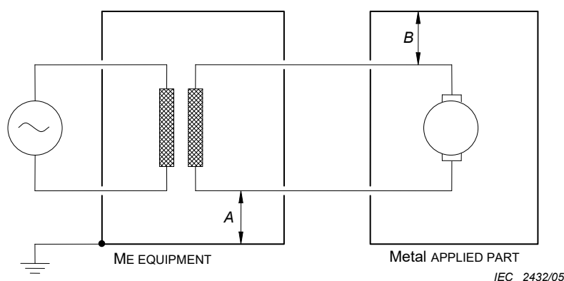
Figure A.10 – Floating circuit
