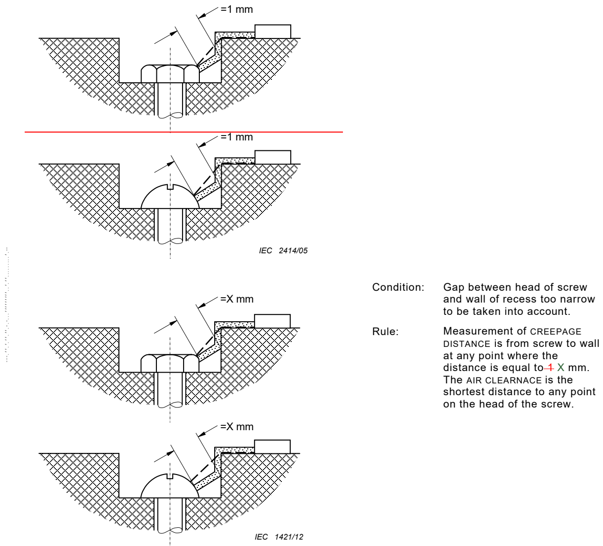
Figure 31 – CREEPAGE DISTANCE and AIR CLEARANCE – Example 10
