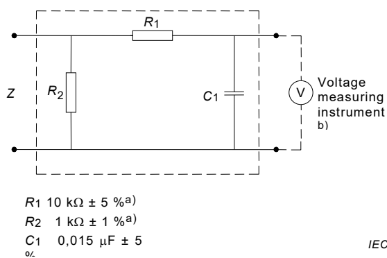
a) Measuring device
