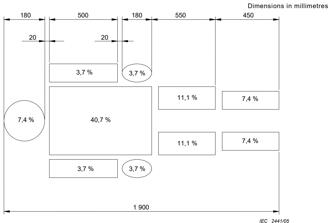
Figure A.18 – Example of human body mass distribution
