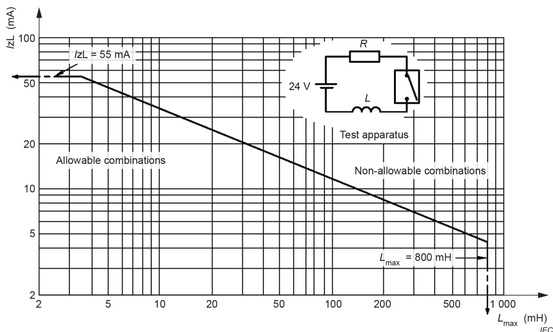
Figure G.6 – Maximum allowable current I_{zL} as a function of the inductance L_{max} measured in an inductive circuit with the most flammable mixture of ether vapour with oxygen
