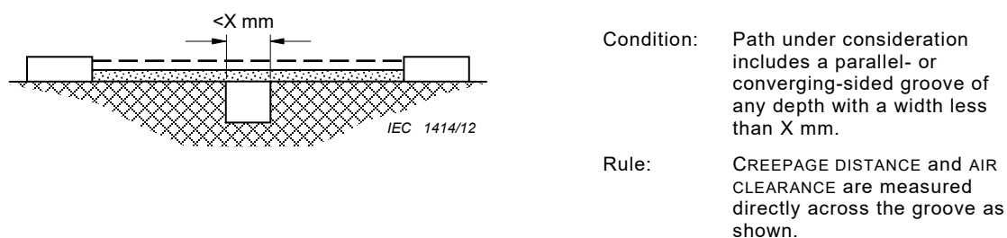
Figure 23 – CREEPAGE DISTANCE and AIR CLEARANCE – Example 2
