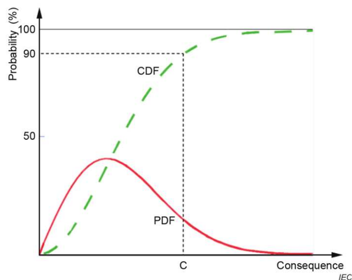
Figure B.18 – Probability distribution function and cumulative distribution function
